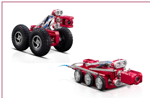
X5-HT Crawler
