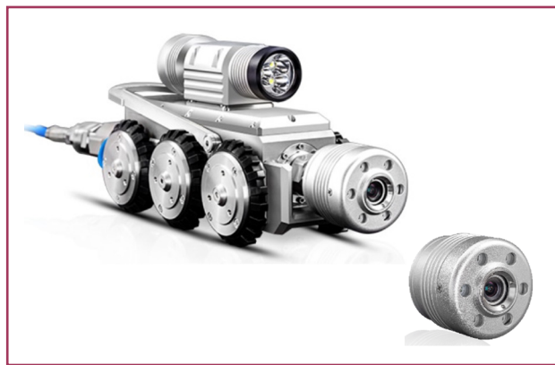
Left - X5-HMA Crawler Right - Axial 50m Camera
